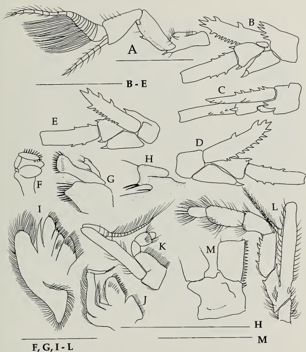
Fig. 2. Pseudopaguristes shidarae , new species: A-D, F-M: holotype male (CBM-ZC 6814), SL = 2.55 mm, off Miyako Is., Okinawa. E: paratype male (CBM-ZC 6815), SL = 2.05 mm, same locality. Left antennule: A, lateral. Left antennal peduncle: B, lateral; C, dorsal; D, mesial. Right antennal peduncle: E, mesial. Left mouthparts: F, mandible, internal; G, maxillule, external; H, same, endopod; I, maxilla, internal; J, first maxilliped, internal; K, second maxilliped, internal; L, third maxilliped, external; M, same, proximal portion, internal. Scales equal 1 mm.
